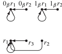
Diagram (c). \text{Cay}(S_\alpha \cup S_\beta, \{(0_\beta, r_1)\})
