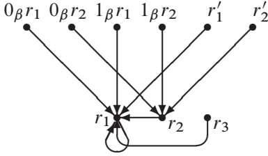
Diagram (b). \text{Cay}(S, \{r_1\})
