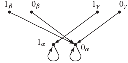
Diagram (g). \text{Cay}(S, \{0_\alpha\})
